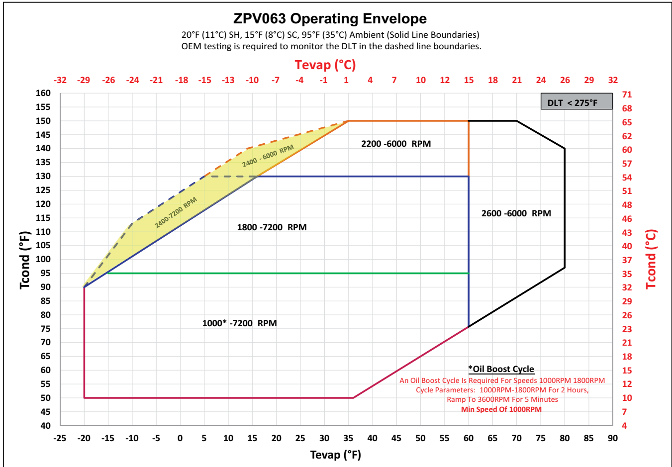
Figure 3 – ZPV063 Operating Envelope
