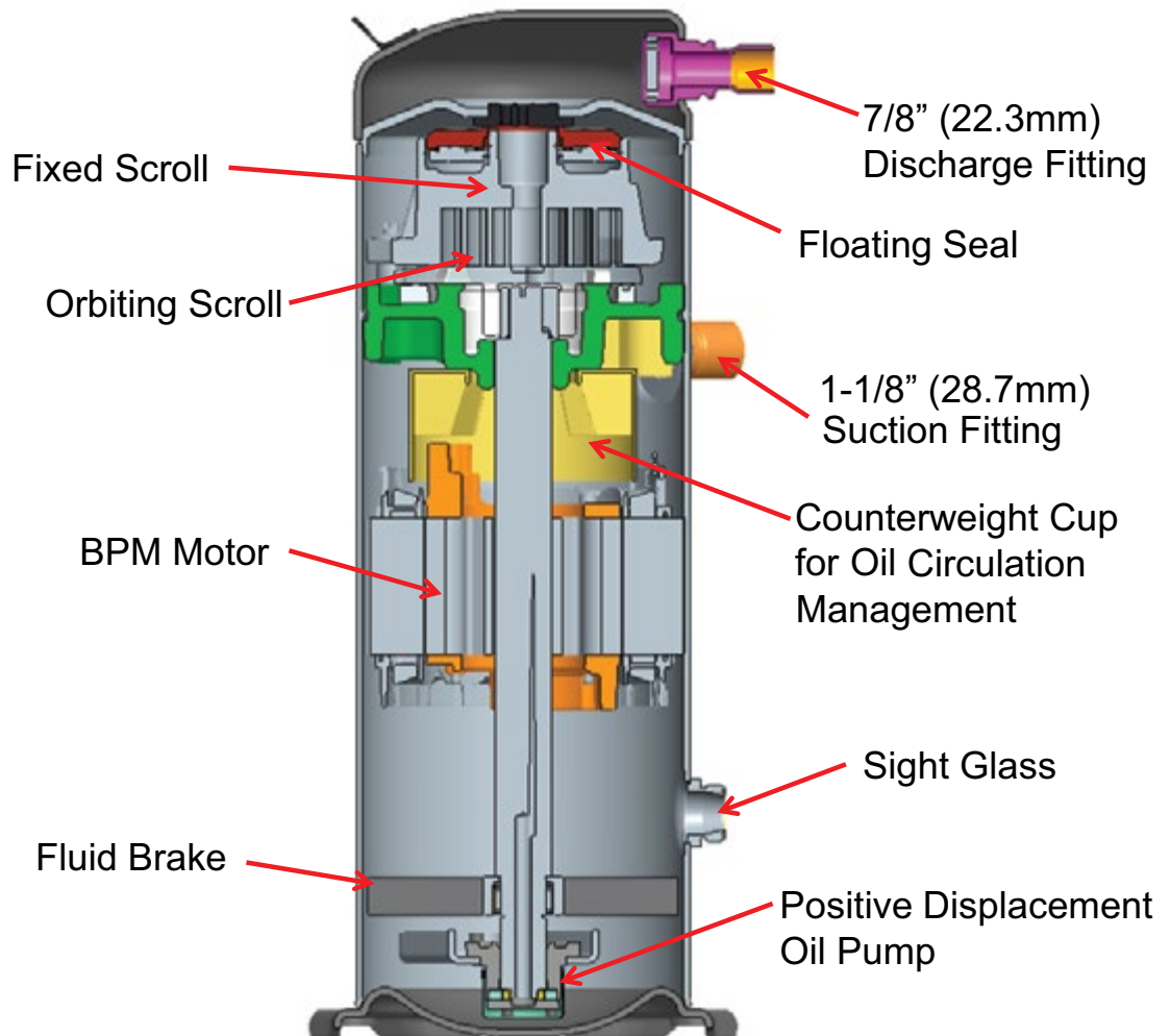
Figure 8 ZPV063 Cross Sectional View
