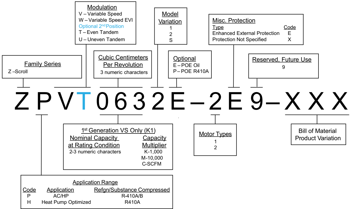
Figure 1 – Compressor Nomenclature
