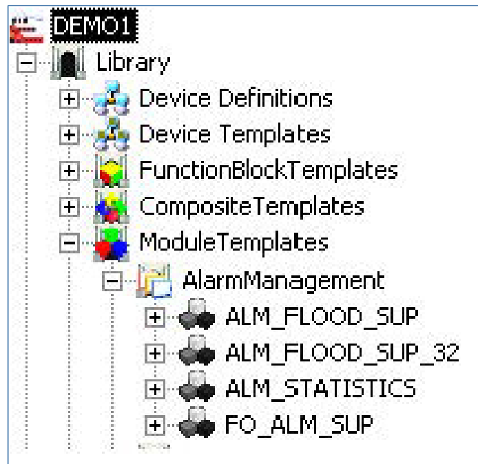
Advanced Alarming Module Templates in the DeltaV Explorer
