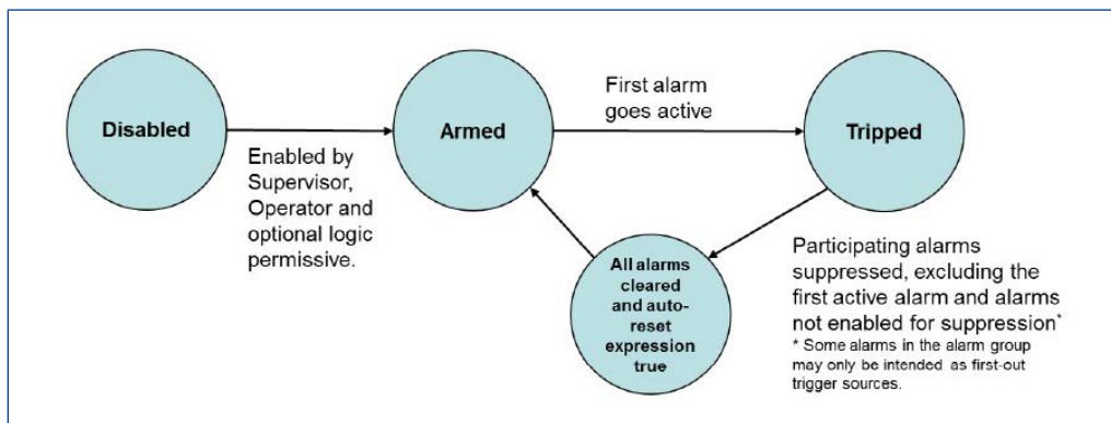
First out module state transition diagram.
