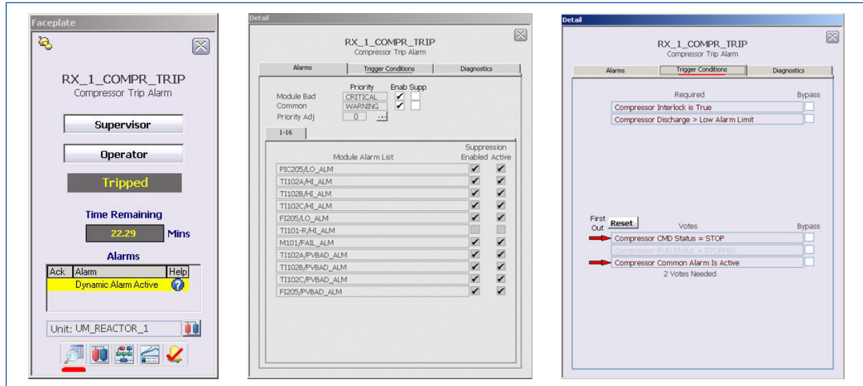
Faceplate and Detail Display for the Alarm Flood Suppression Module.
