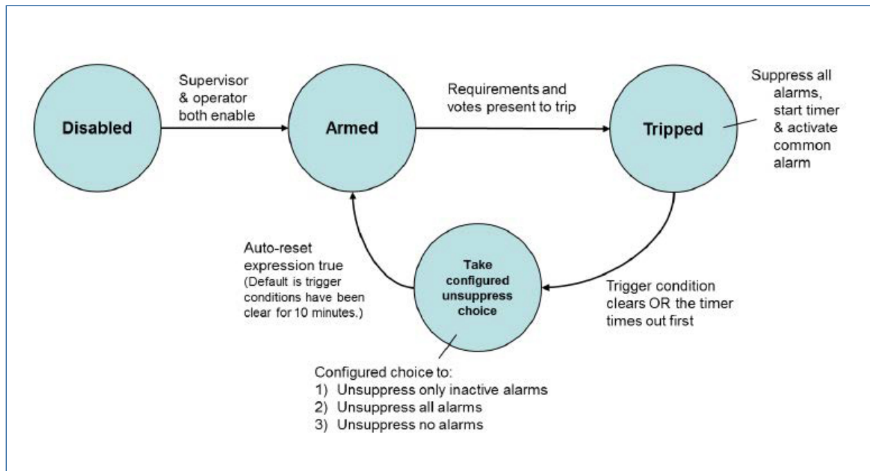
Alarm Flood Suppression module state transition diagram.
