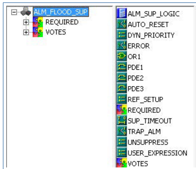
The ALM_FLOOD_SUP module uses composite blocks for the required and voting (trigger) conditions.
