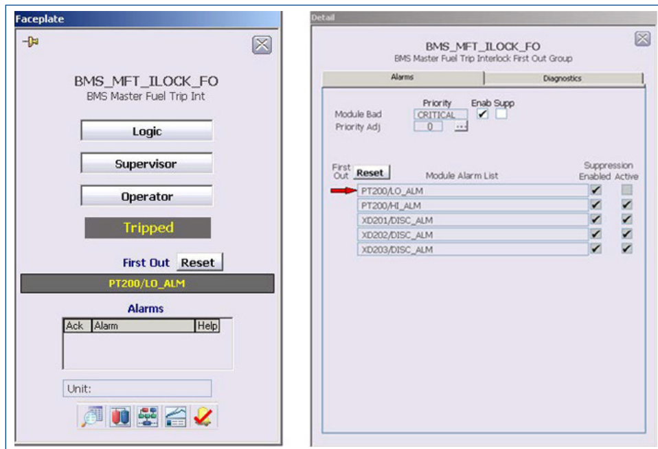
Faceplate and Detail Display for the First-Out Alarming Module.
