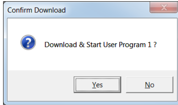
Figure 2-8. Confirm Download
