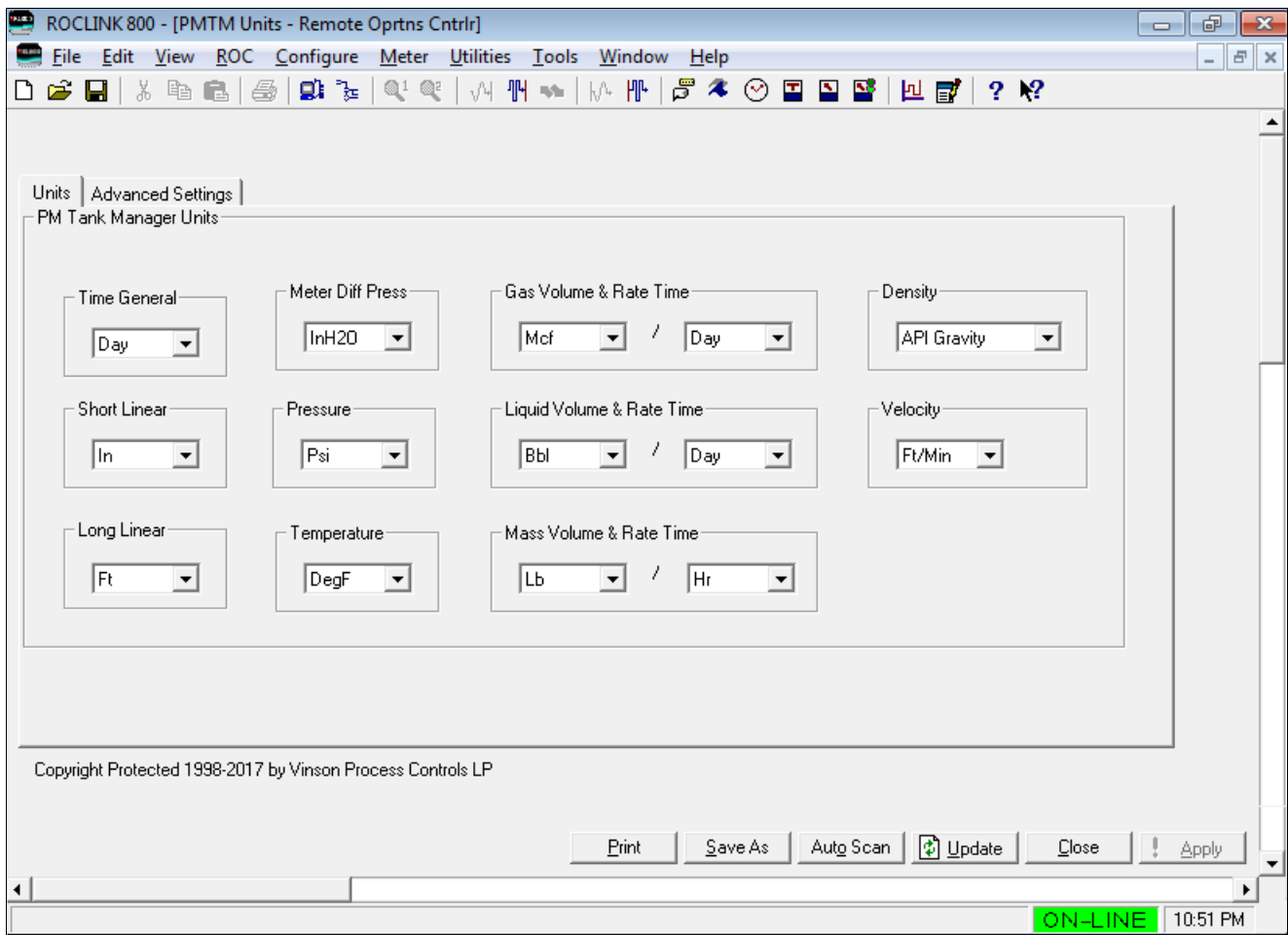
Figure 3-2. Unit Screen
