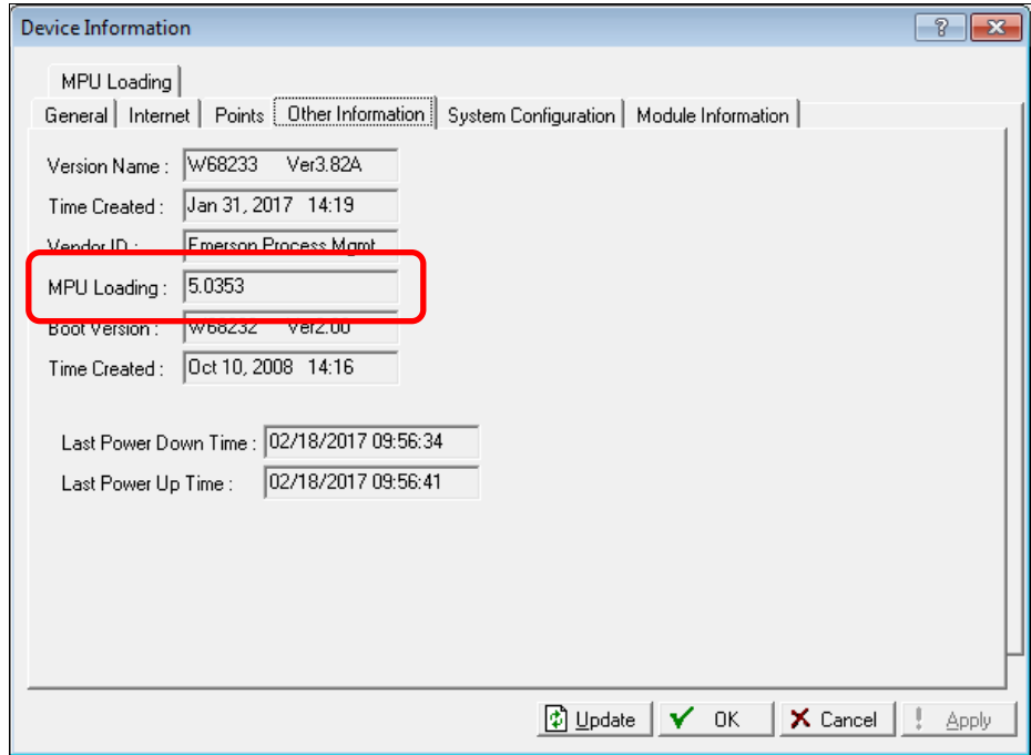
Figure 2-26. MPU Loading
