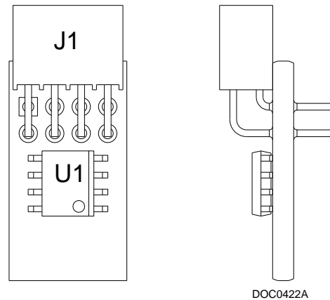
Figure 1-1. License Key
