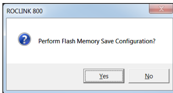
Figure 3-26. Save Verification
