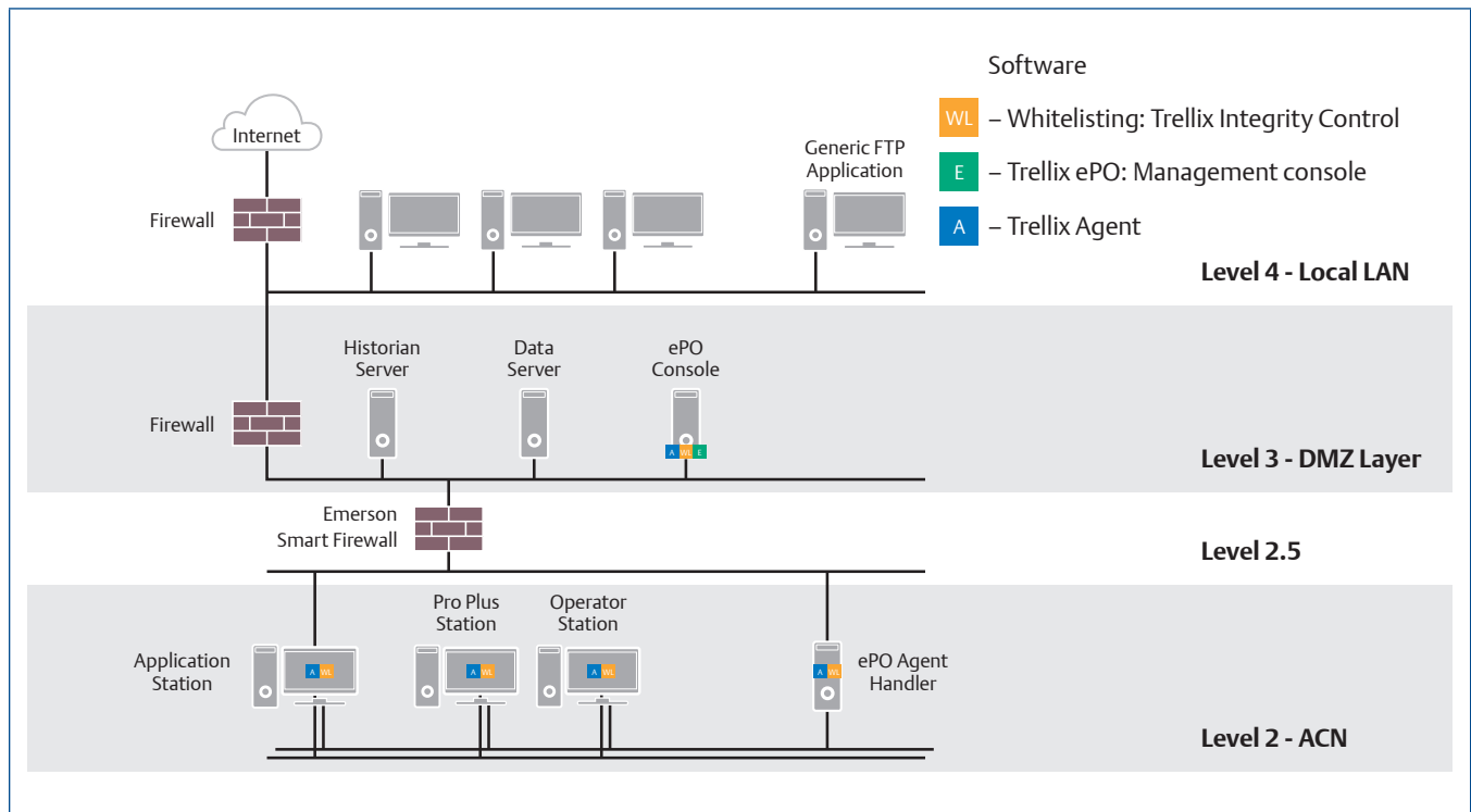
Example reference architecture for Application Whitelisting for DeltaV Systems on a typical DeltaV network.
