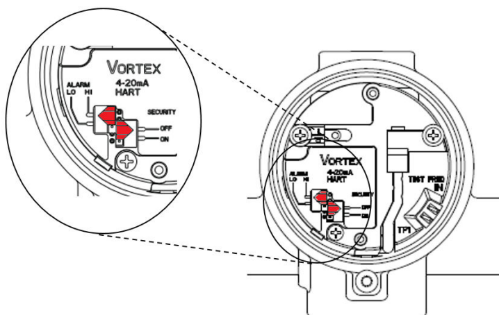
Figure 2-5: ALARM jumper location without (M5) optional display
