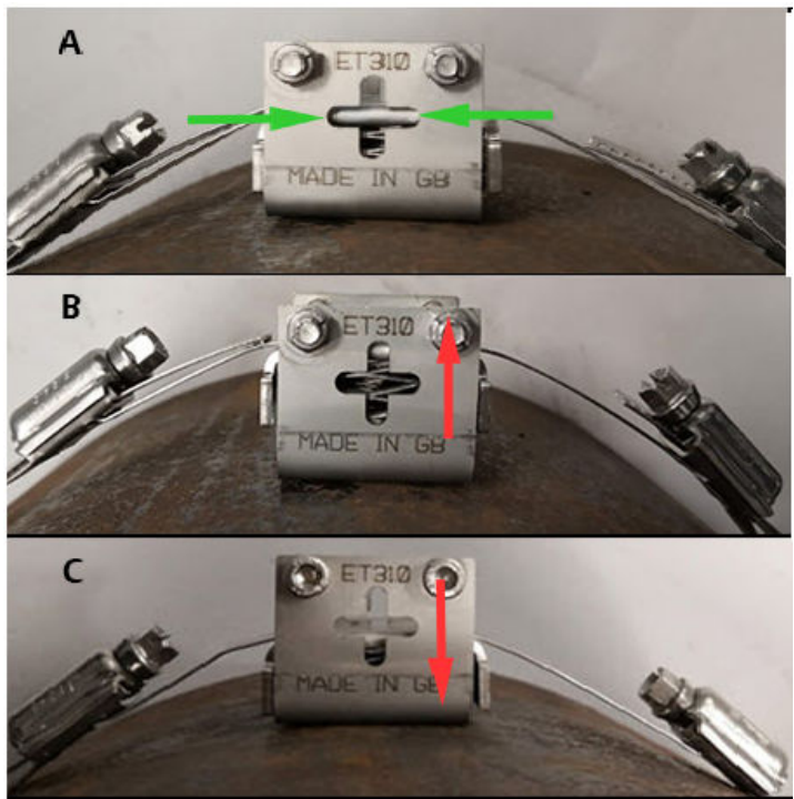
Figure 3-5: Alignment examples
