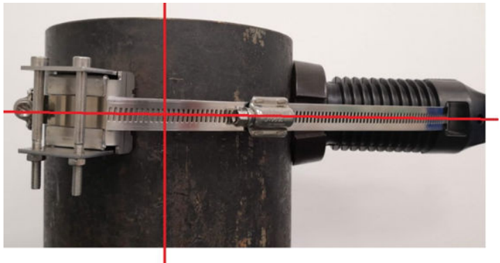
Figure 3-4: Correct strap alignment
