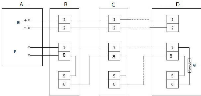
Figure 2-5: Typical wiring for four-wire controllers
