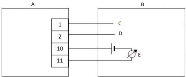
Figure 2-7: Sink four-wire
