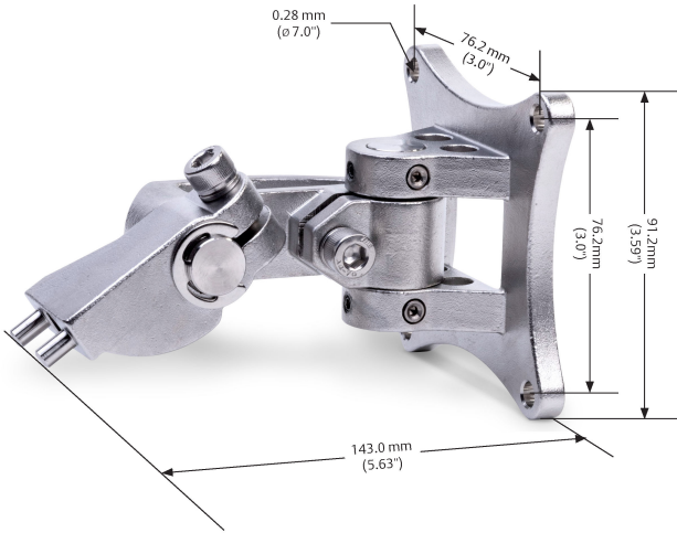
Figure 2-3: Tilt mount with dimensions
