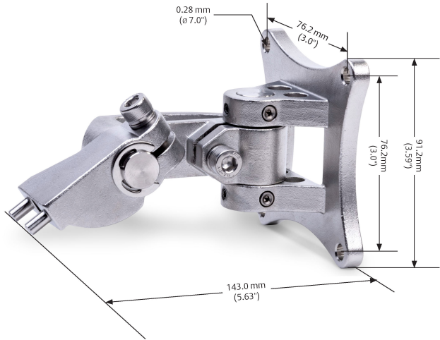
Figure 2-9: Tilt mount
