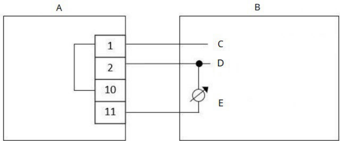
Figure 2-8: Source three-wire
