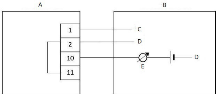
Figure 2-6: Non-isolated sink (three wires)
