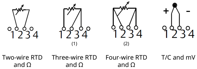
Figure 3-1: Sensor Connections
