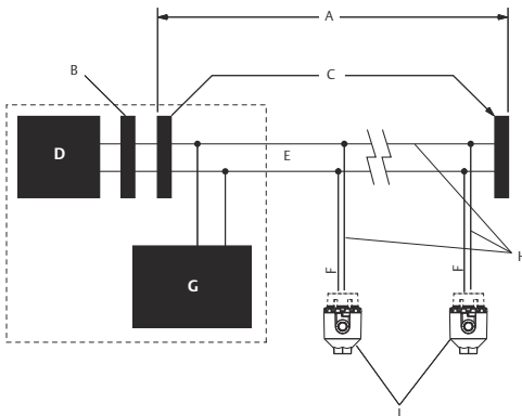
Figure 3-2: Typical Configuration for PROFIBUS Networking
