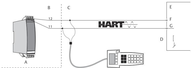
Figure 4-1: HART communicator
