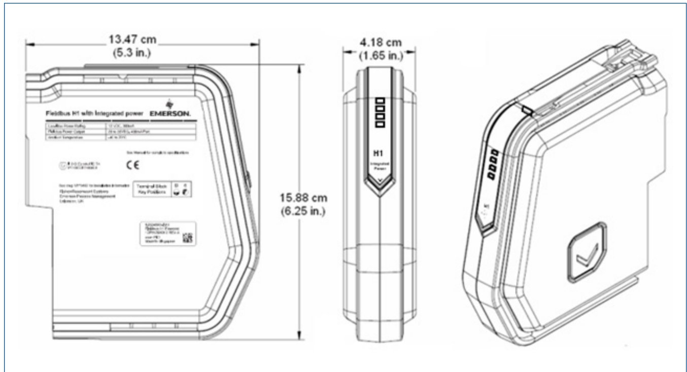
S-series H1 interface with integrated power dimensions.
