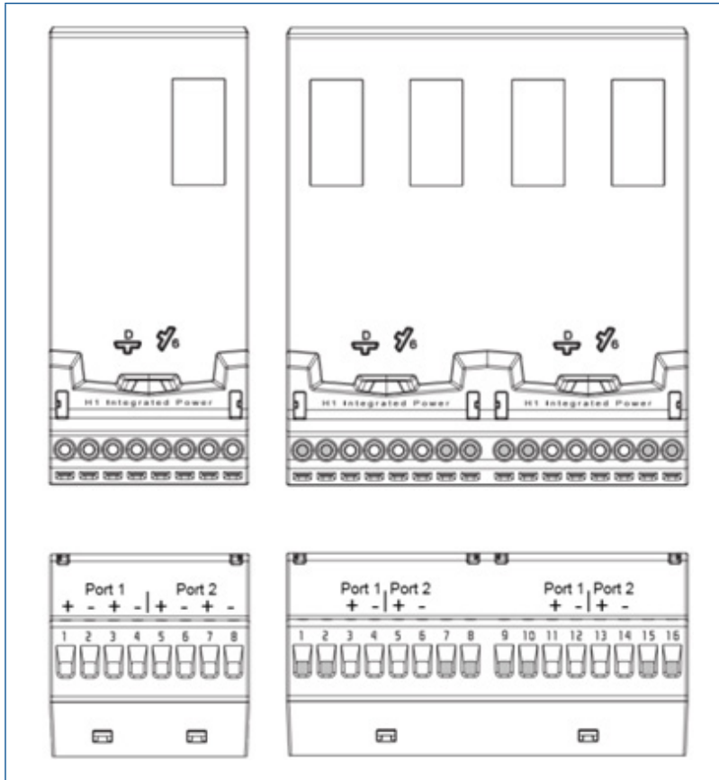
S-series H1 with Integrated power Terminal Blocks.
