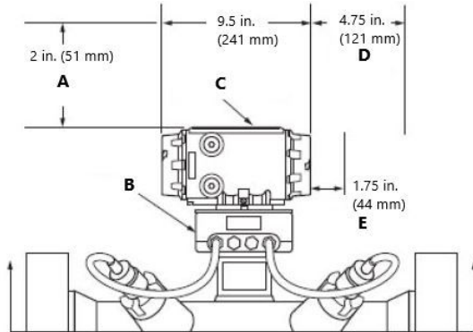
Figure 6: In-line Position of Enclosure Housing
