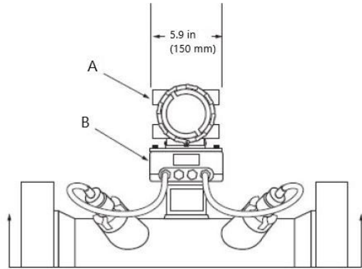
Figure 7: Optional Position of Enclosure Housing (8)
