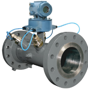
Figure 4: Optional larger, retrofit electronics enclosure on JuniorSonic 3412 meter (no optional display available)
