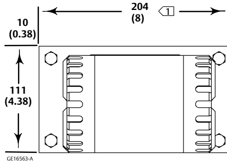
MOUNTING BRACKET DIMENSIONS FOR FISHER 585CLS ACTUATORS WITH A 152 mm (6-INCH) CHANNEL
