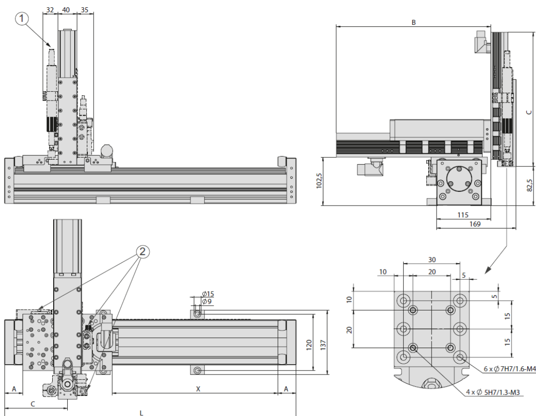
Fig. 10 Dimensioned drawing EPS midi XYZ
