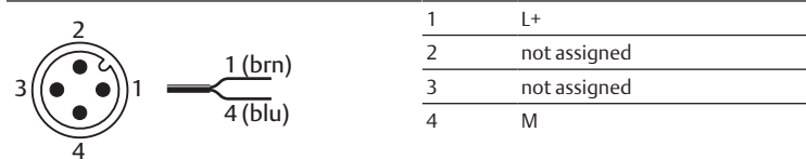
Fig. 1: Sensor porting configuration
