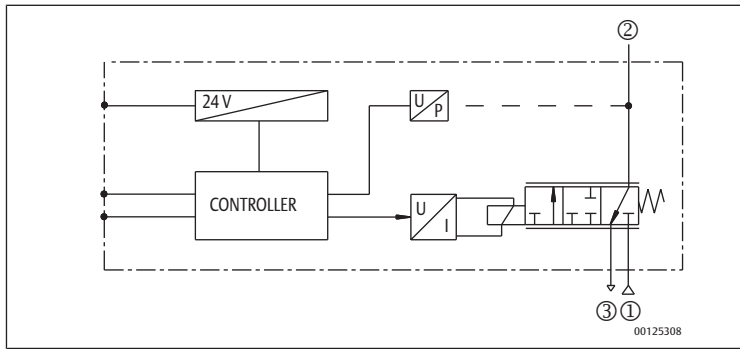
Fig. 6: Functional diagram
