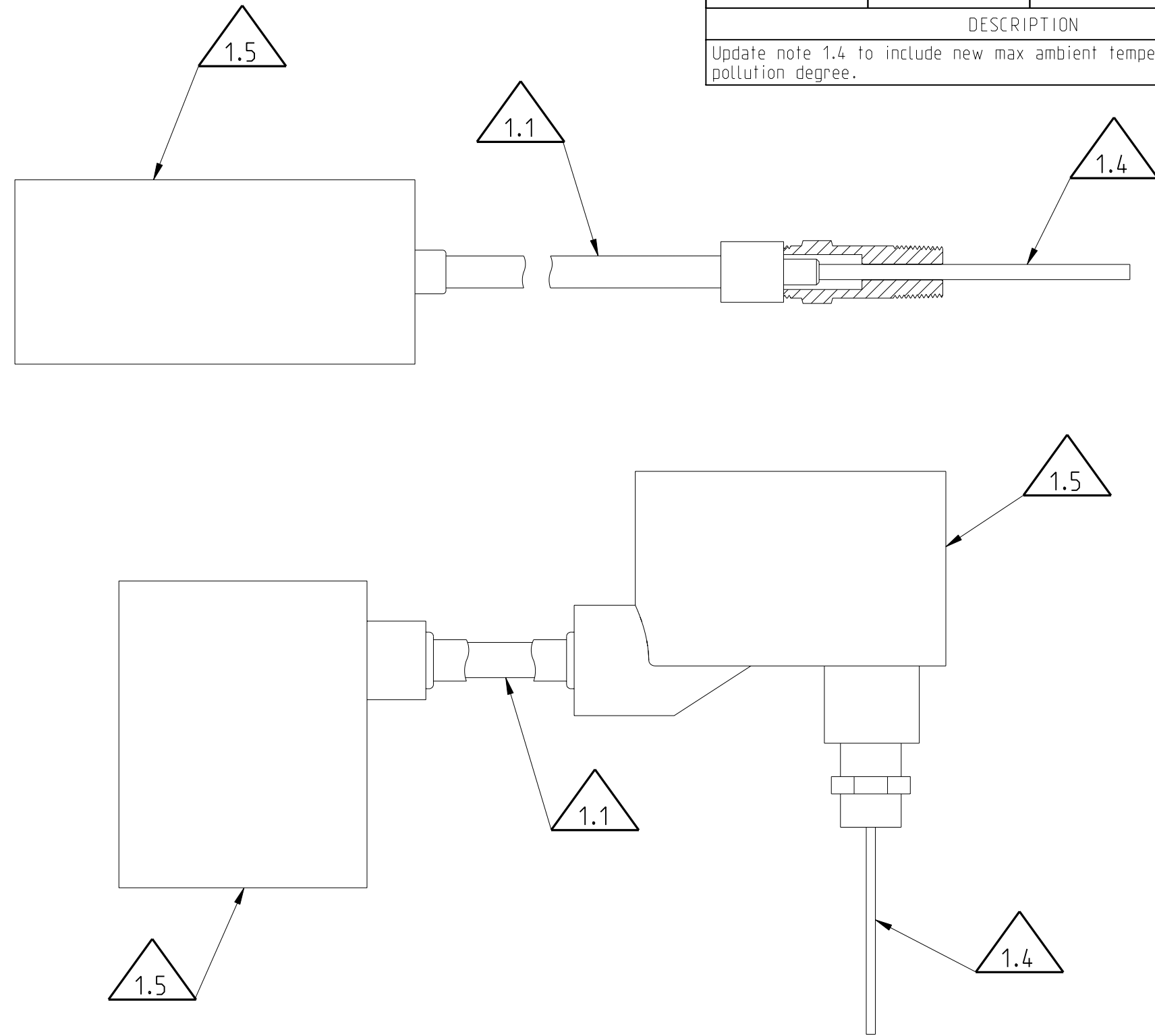
EXPLOSIONPROOF REMOTE MOUNT CONFIGURATIONS
