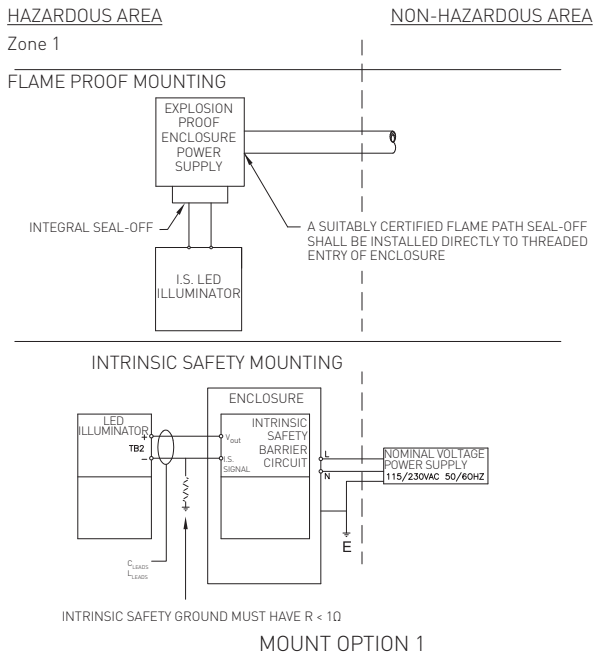
FIGURE 6B Control drawing for ATEX/IECEx
