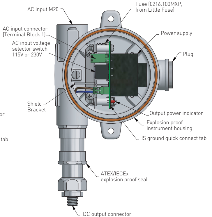
FIGURE 5C Wiring installation - ATEX/IECEX locations
