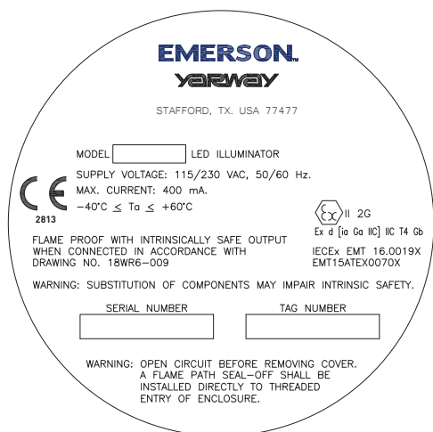
FIGURE 7C Nameplate - ATEX/IECEX
