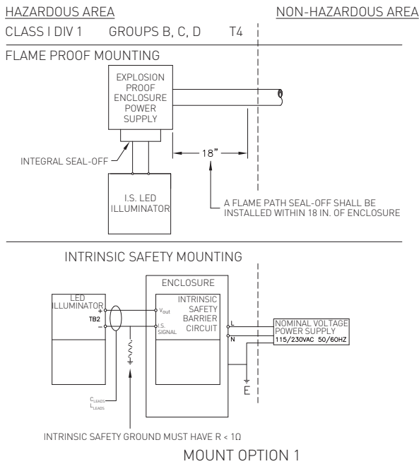
FIGURE 6A Control drawing for division locations
