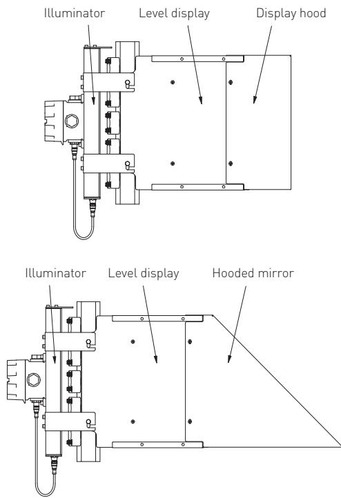
FIGURE 4 Accessories views
