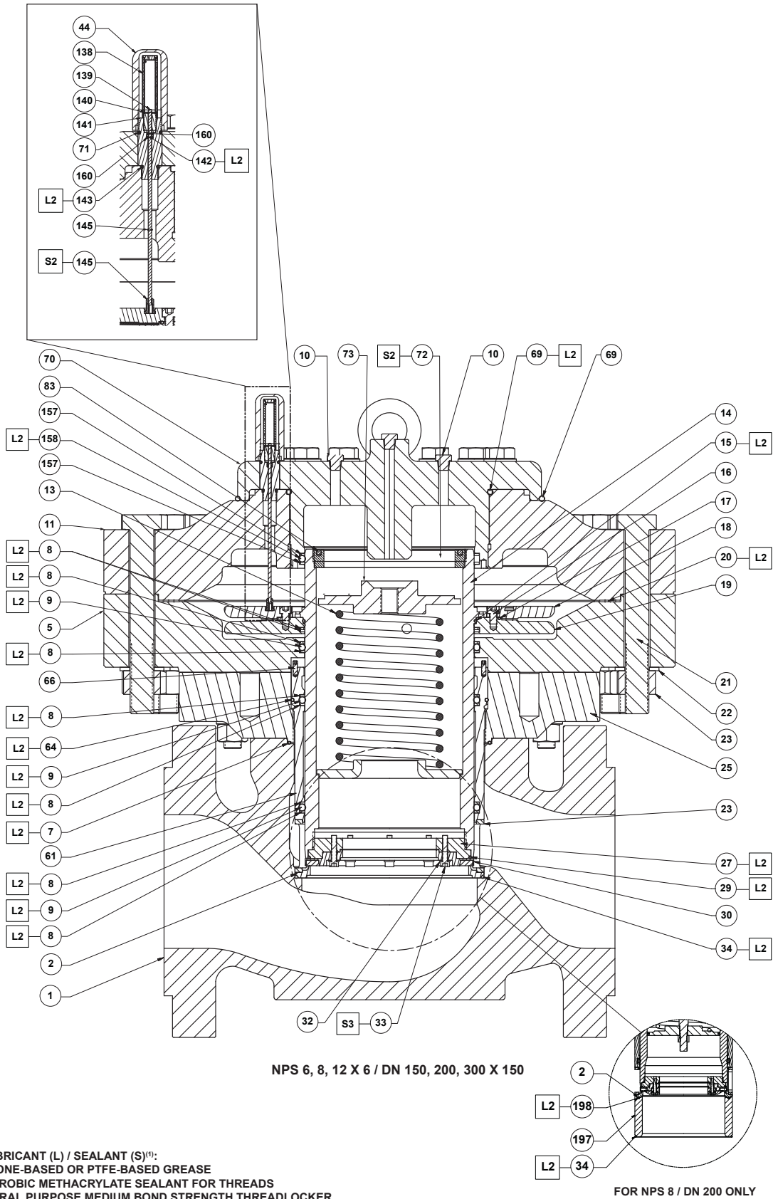
Figure 4. Type EZH Main Valve Assembly (continued)
