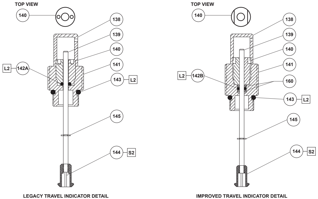
Figure 4. Type EZH Main Valve Assembly (continued)
