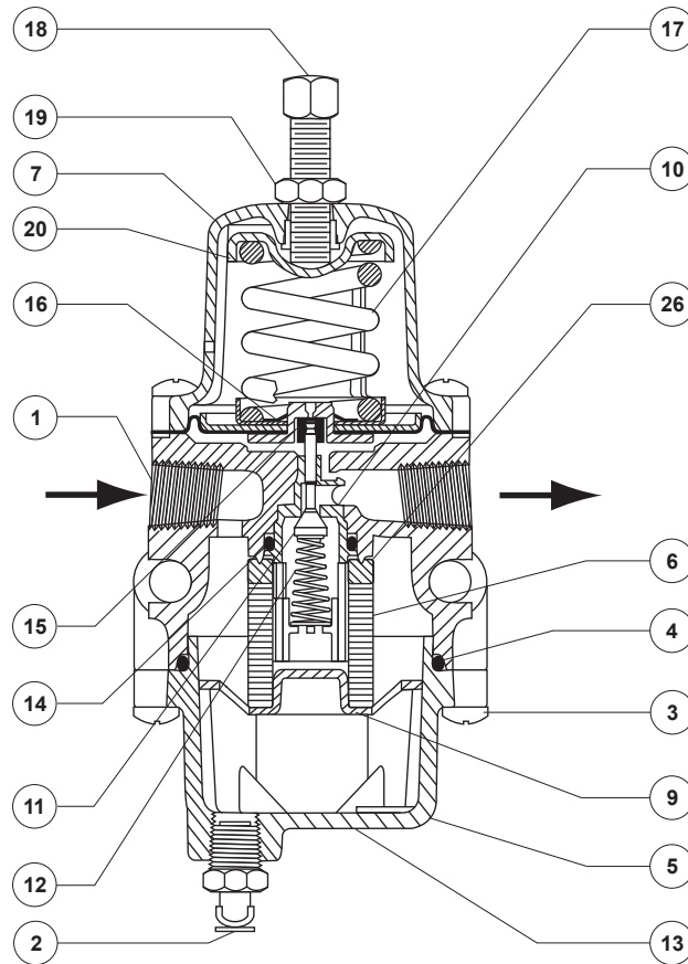
Figure 2. 67CF Series Assembly Drawings
