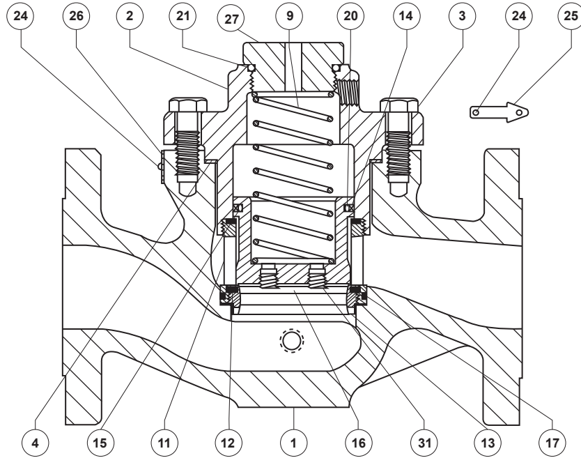
COMPLETE CAST IRON MAIN VALVE ASSEMBLY
