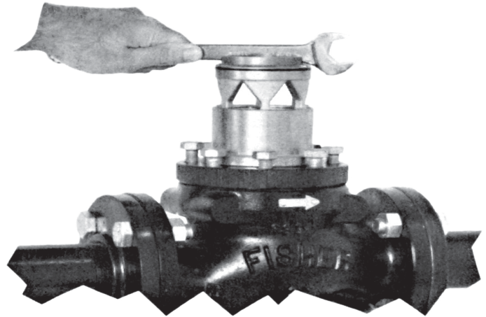
Figure 9. Seat Ring and/or Cage Removal Using Body as a Holding Fixture
