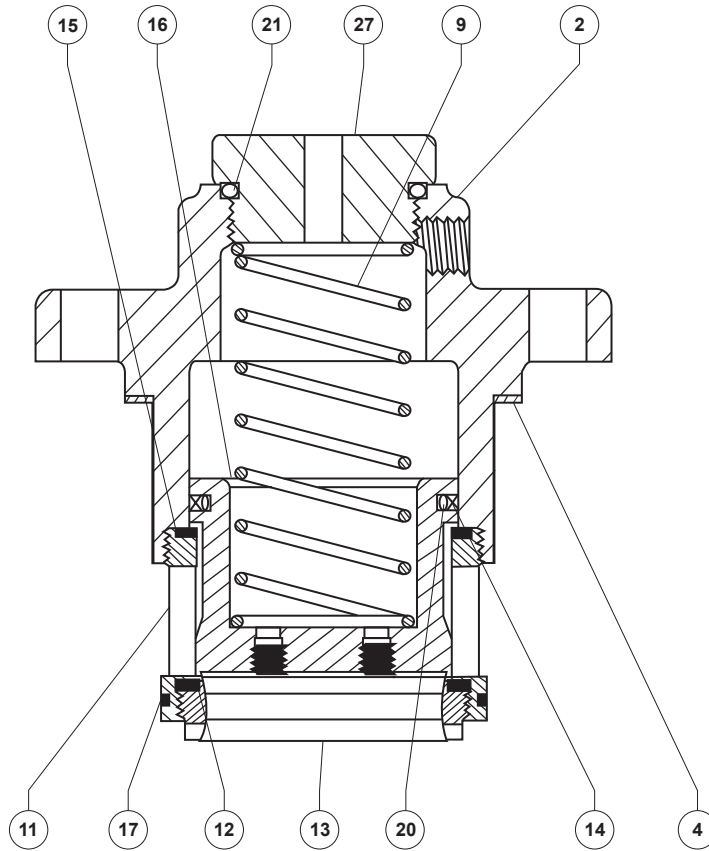
QUICK-CHANGE TRIM PACKAGE ASSEMBLY
