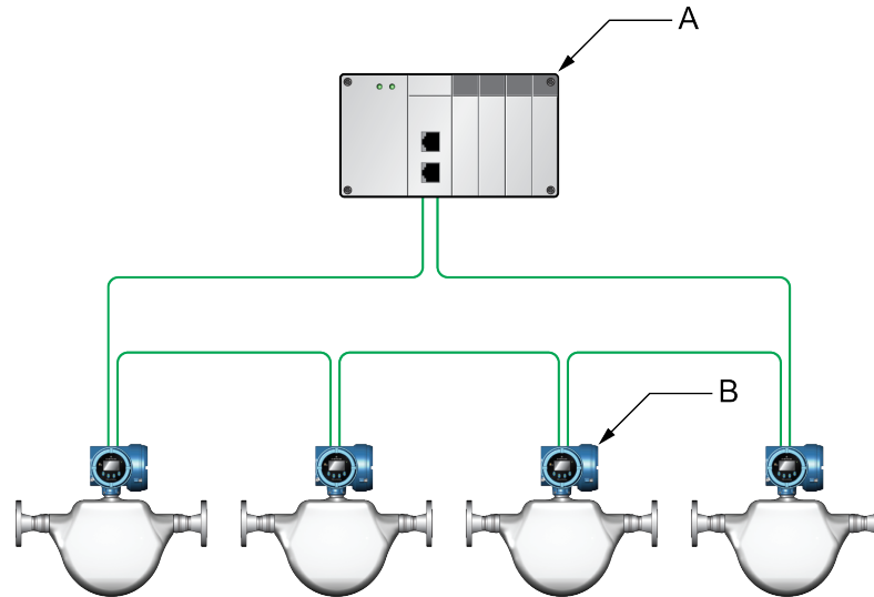
Figure 2-2: 5700 ring network
