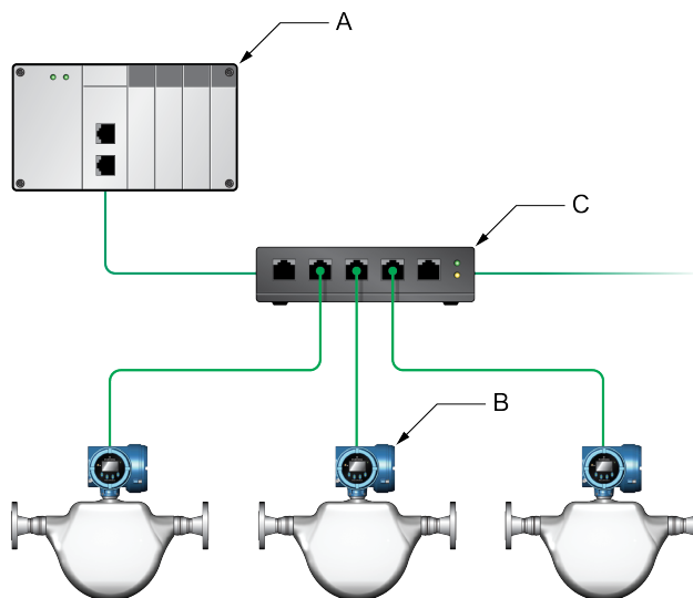
Figure 2-1: 5700 star network
