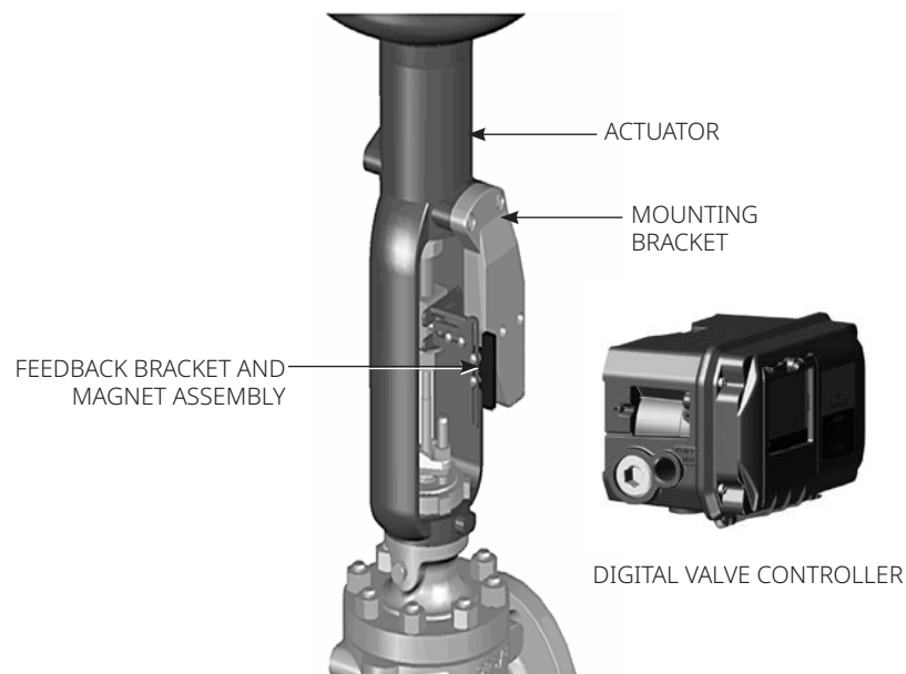
Figure 2. DVC7K Magnetic Assembly
