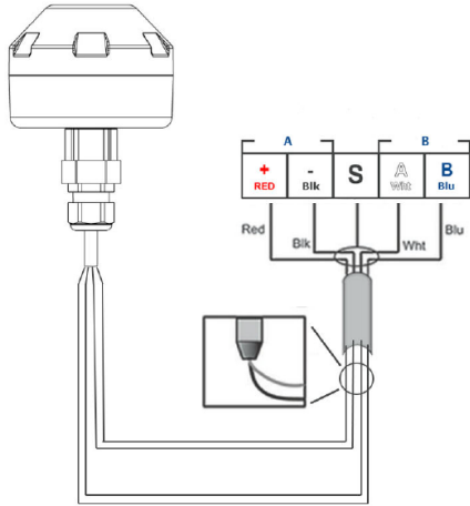
781 Power and Data Wiring
