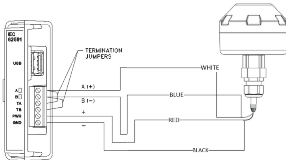
IEC 62591 Module Power and Data Wiring to 7815
