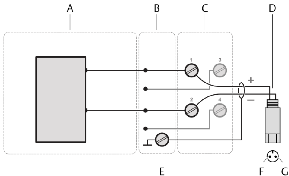
Figure 3-3: Sensor connection
