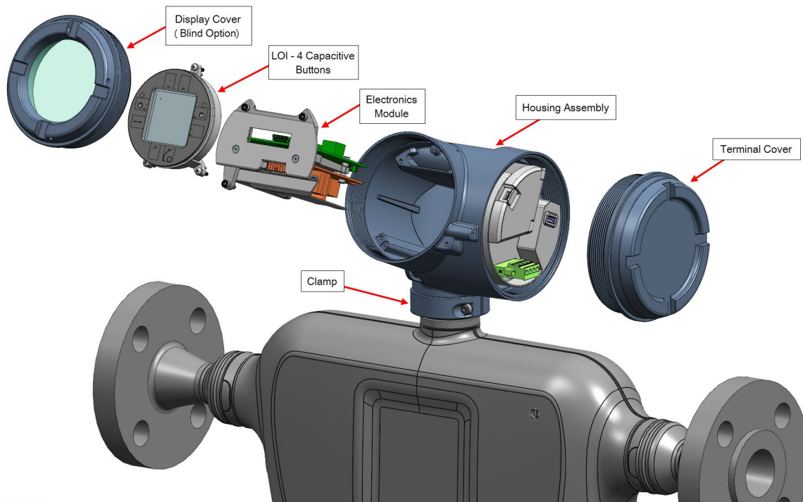
Figure 1 4200, Parts included in the FMEDA
