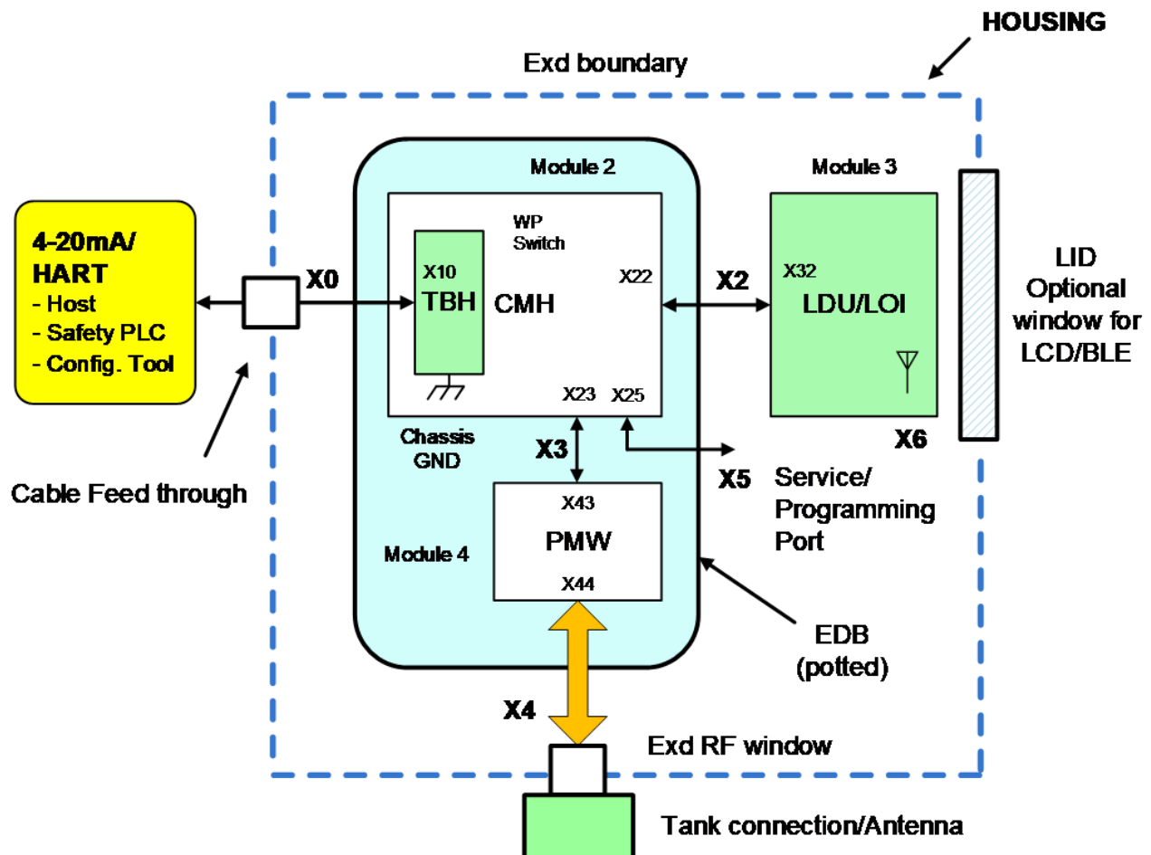
Figure 1 3408, Parts included in the FMEDA
