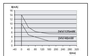
Current-time diagram (24V/46mW - 24V/125mW) Diagramme courant-temps (24V/46mW - 24V/125mW) Strom-Zeit (24V/46mW - 24V/125mW)
