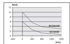
Current-time diagram (6V/3mW-8V/22mW) Diagramme courant-temps (6V/3mW - 8V/22mW) Strom-Zeit (6V/3mW - 8V/22mW)
