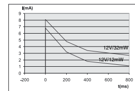
Current-time diagram (12V/12mW-12V/32mW) Diagramme courant-temps (12V/12mW - 12V/32mW) Strom-Zeit (12V/12mW - 12V/32mW)
