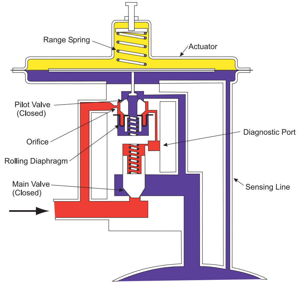
Closed Pilot
