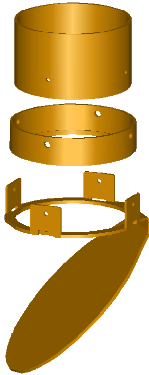
Picture 3. Reflector is mounted to the pipe with the Ring marked DN 100.
