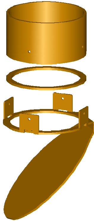
Picture 2. Reflector is mounted to the pipe with the Ring marked 4" SCH 40.
