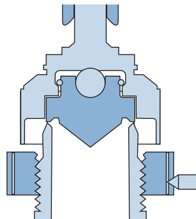
TYPICAL LIQUID RELIEF VALVE DISC
