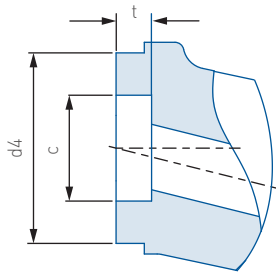
Socket weld end
