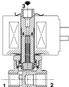
NO function (1/4)
