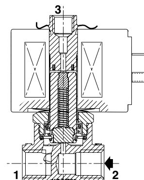
NC function (1/4)
