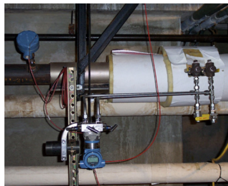
Rosemount Orifice Plate (check meter) installed downstream of the Rosemount Orifice Flow Meter
