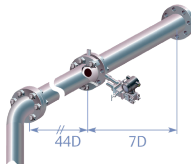
Comparison of required straight pipe lengths (Conditioning Orifice Plate vs. Traditional Orifice Plate)
