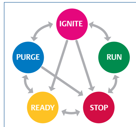
The different states and transitions for a burner are represented by a state transition diagram in the DeltaV SIS system.
