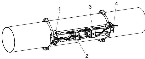
Abb. 7.57: Sensoren in Schiene
